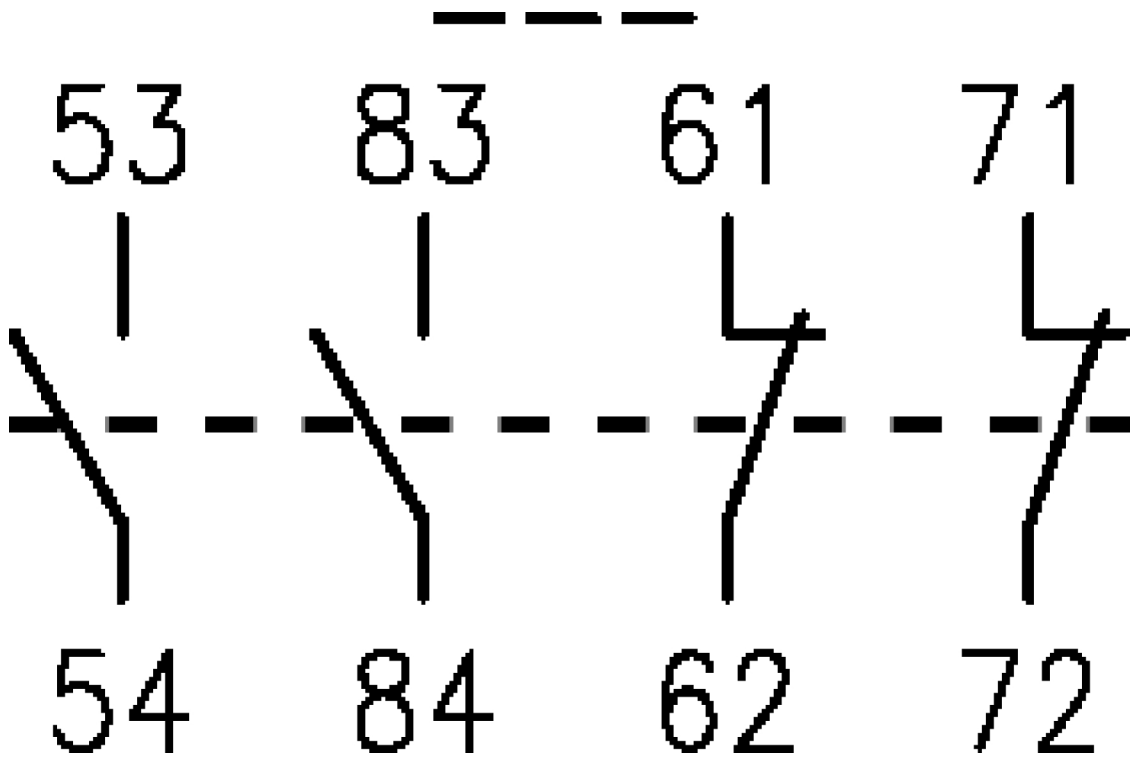
Connection / Wiring Diagram
