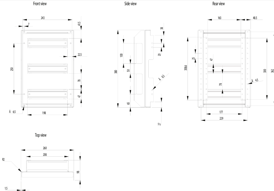
Dimension Diagram
